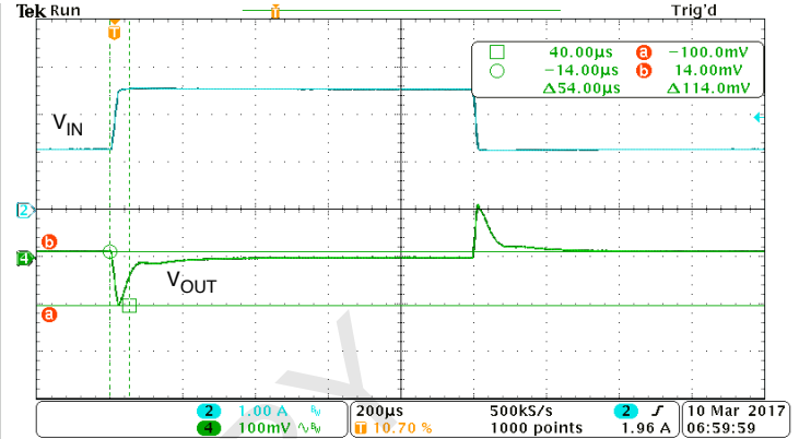
UNITS ARE PER DIVISION SMHF4205S LOAD TRANSIENT 50-100-50% FIGURE 6
