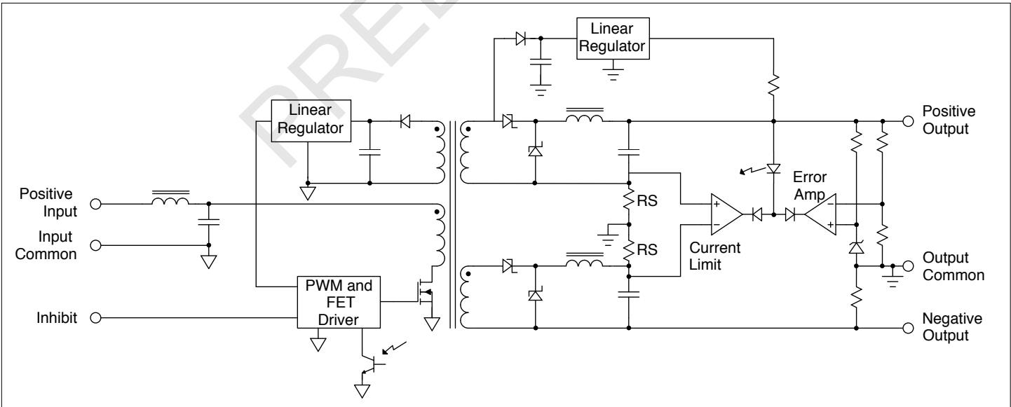
FIGURE 2: SMHF42 DUAL OUTPUT, BLOCK DIAGRAM
