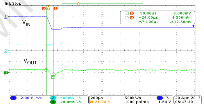
UNITS ARE PER DIVISION SMHF4205S LINE TRANSIENT 55 TO 53 VIN FIGURE 8
