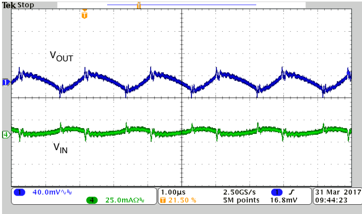
UNITS ARE PER DIVISION, 42 VIN, 100% LOAD SMHF4215D INPUT AND OUTPUT RIPPLE REPRESENTATIVE OF ALL SMHF42 FIGURE 5
