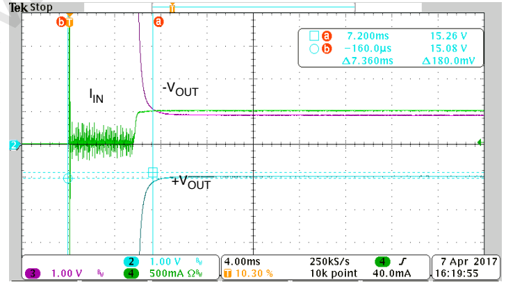
UNITS ARE PER DIVISION SMHF4215D START-UP DELAY FIGURE 16
