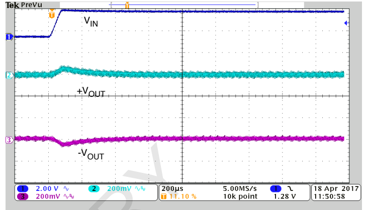
UNITS ARE PER DIVISION SMHF4215D LINE TRANSIENT 53-55 VIN FIGURE 14
