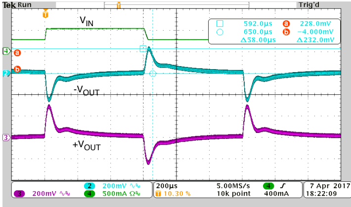
UNITS ARE PER DIVISION SMHF4215D LOAD TRANSIENT 50-100-50% FIGURE 13
