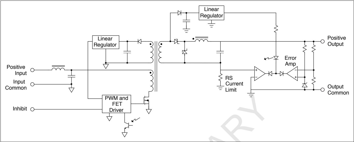
FIGURE 1: SMHF42 SINGLE OUTPUT, BLOCK DIAGRAM
