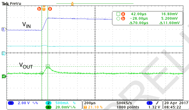
UNITS ARE PER DIVISION SMHF4205S LINE TRANSIENT 53 TO 55 VIN FIGURE 7
