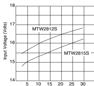
MTW2812S and MTW2815S Low Line Dropout FIGURE 6
