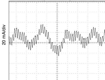
10 \mu s/div MOR2815S Input Ripple (Iin)
