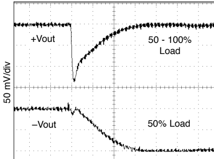
MOR2805D Step Load Response
