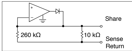
FIGURE 8: SHARE
