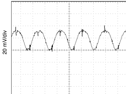
1 \mu s/div MOR2815S Output Ripple (Vout)
