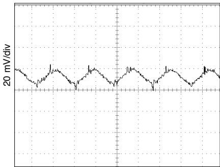
1 μs/div 80% Load MOR2805S Output Ripple (Vout)
