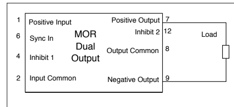
FIGURE 11: SPANNED OUTPUTS – DUAL MODEL
