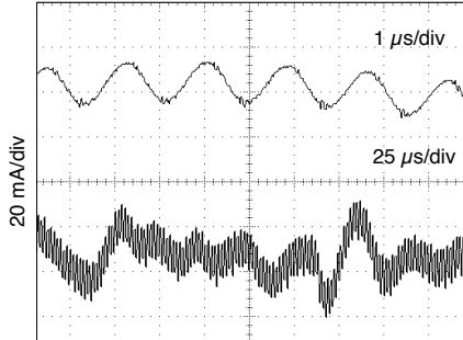
80% load each output MOR2805D Input Ripple (lin)
