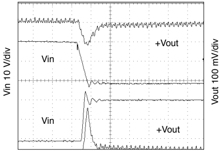
MOR2812D Step Line Response
