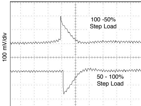
100 μs/div MOR2805S Step Load Response
