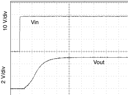
2.5 ms/div All combinations of line and load MOR2805S Start-up Response
