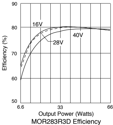
MOR283R3D Efficiency
