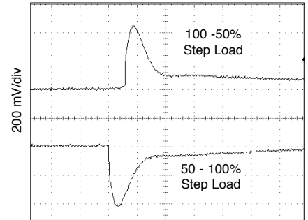
100 \mu s/div MOR2815S Step Load Response
