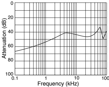
MOR2805S Audio Rejection
