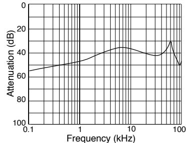
MOR2815S Audio Rejection
