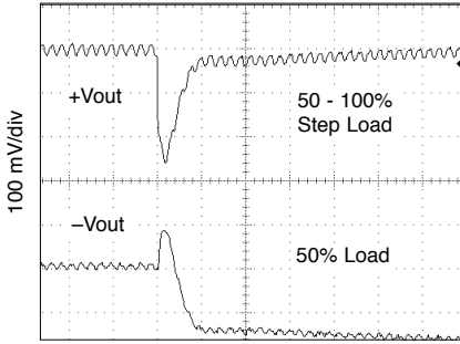
MOR2812D Step Load Response
