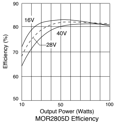
MOR2805D Efficiency
