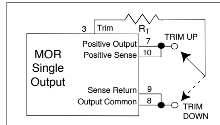
FIGURE 2: TRIM – SINGLE
