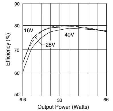
MOR283R3S Efficiency
