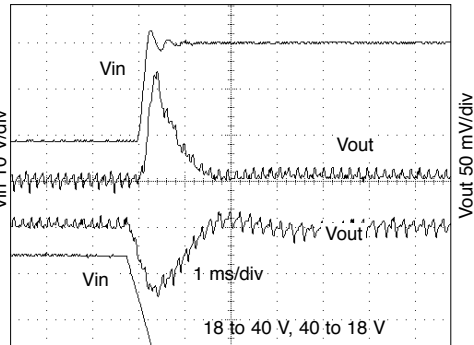
MOR2805S Step Line Response
