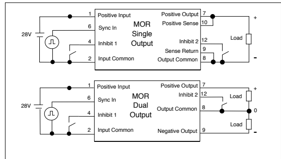
FIGURE 10: TYPICAL CONNECTIONS
