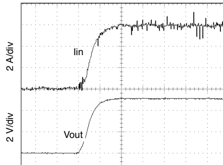
5 ms/div With and without 470 μF cap. load MOR2805S Inhibit Release Inrush Current
