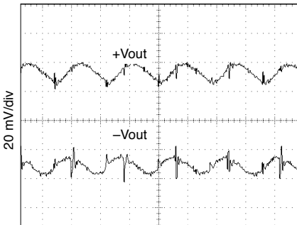
80% load each output MOR2805D Output Ripple (±Vout)
