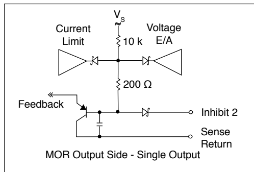
FIGURE 5: INHIBIT 2
