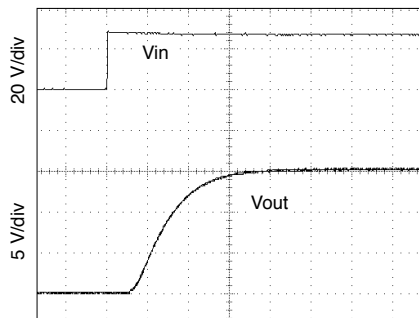
2.5 ms/div All combinations of line and load MOR2815S Start-up Response
