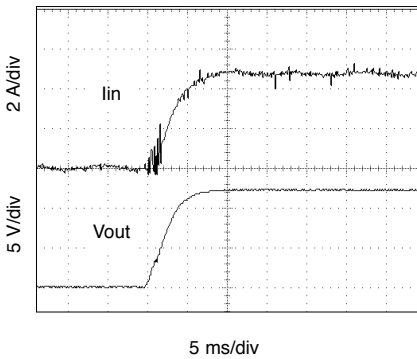
MOR2812D Inhibit Release Inrush Current
