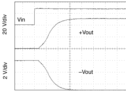
MOR2805D Start-up Response
