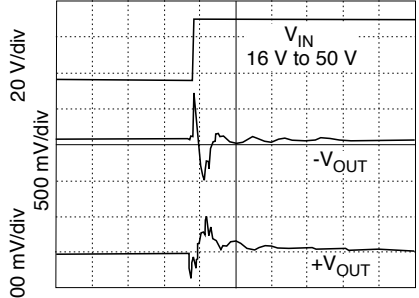
40 \mu s/div STEP LINE RESPONSE MHV2815D
