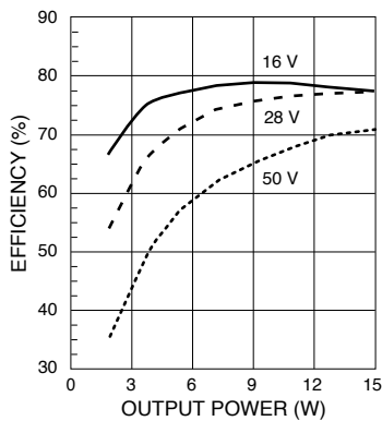
MHV2805S EFFICIENCY
