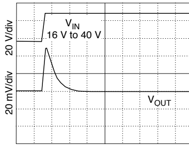
400 \mu s/div STEP LINE RESPONSE MHV2805S
