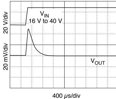
400 \mu s/div STEP LINE RESPONSE MHV2805S
