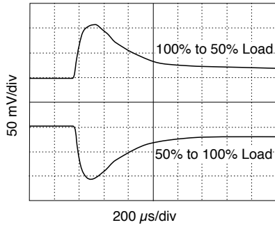
200 \mu s/div STEP LOAD RESPONSE MHV2805S
