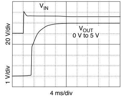
4 ms/div TURN ON RESPONSE MHV2805S
