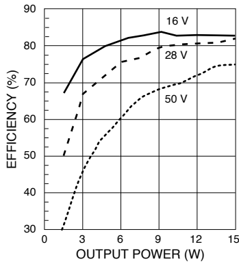
MHV2812S EFFICIENCY
