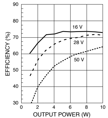
MHV283R3S EFFICIENCY
