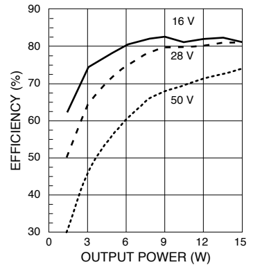
MHV2815S EFFICIENCY
