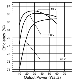
MFW28515T Efficiency vs Line & Load
