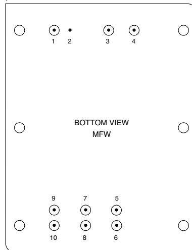
FIGURE 2: PIN OUT
