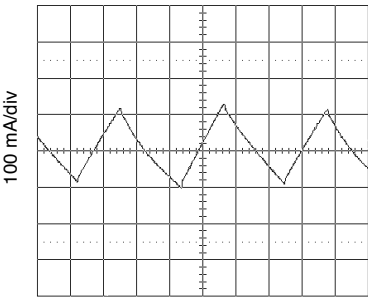
3.3 V IN , 1.2 V OUT , 5 A load MFP0507S Input Ripple (I IN ) FIGURE 12
