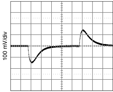
3.3 V IN , 1.2 V OUT , 5 A load MFP0507S Load Transient FIGURE 16
