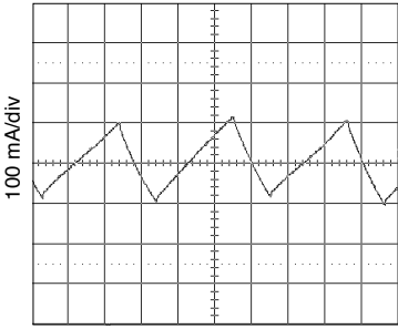
5 V IN , 3.3 V OUT , 5 A load MFP0507S Input Ripple (I IN ) FIGURE 13
