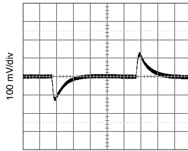
5 V IN , 3.3 V OUT , 5 A load MFP0507S Load Transient FIGURE 17
