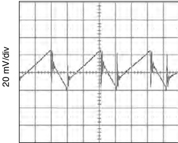
5 V IN , 3.3 V OUT , 5 A load MFP0507S Output Ripple FIGURE 15
