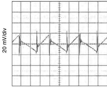
3.3 V IN , 1.2 V OUT , 5 A load MFP0507S Output Ripple FIGURE 14
