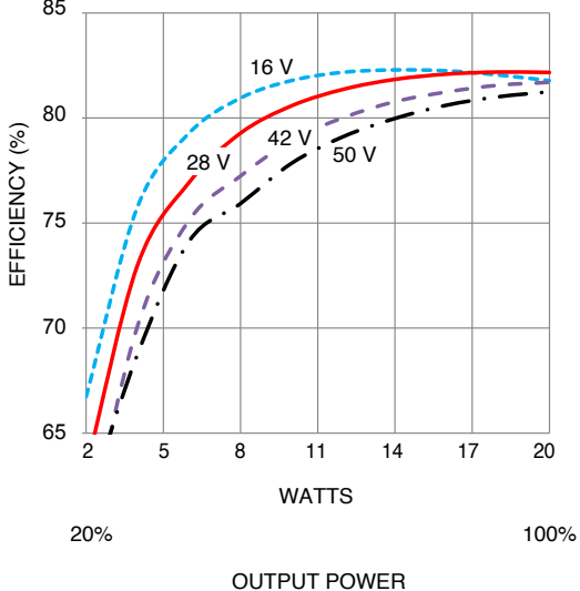
MFK2805S EFFICIENCY
