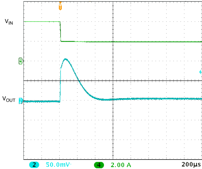
UNITS ARE PER DIVISION MFK2805S STEP LOAD 100% - 50%
