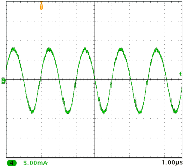
UNITS ARE PER DIVISION MFK2815D INPUT RIPPLE
