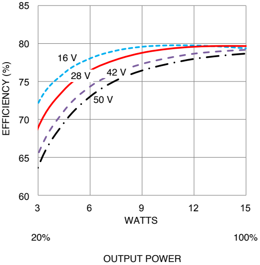
MFK283R3S EFFICIENCY
