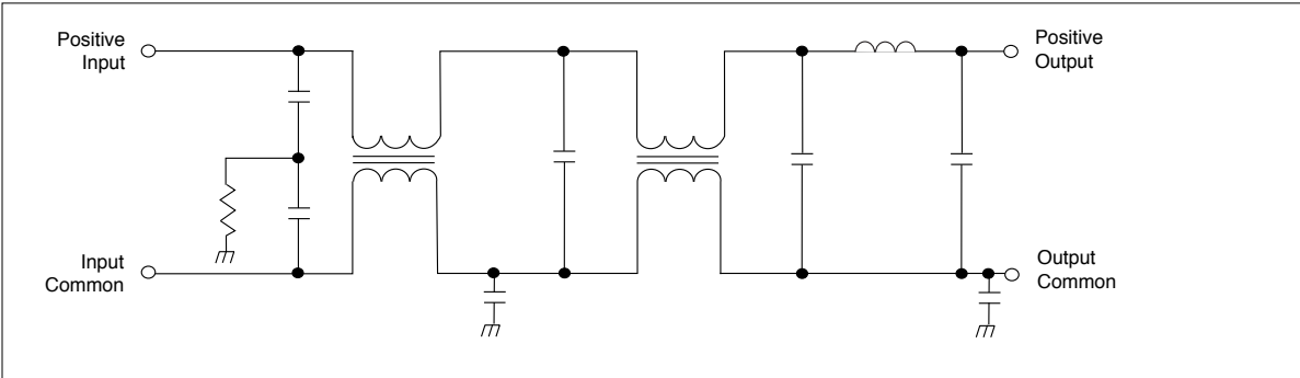
FIGURE 2: SCHEMATIC - FMCE-0328
